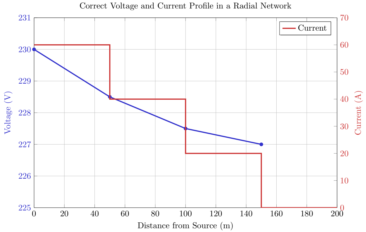
Figure 1: A physically correct plot showing voltage drop in a radial network. As the current (red) decreases in steps, the slope of the voltage profile (blue) becomes progressively flatter, indicating a smaller voltage drop per meter.
